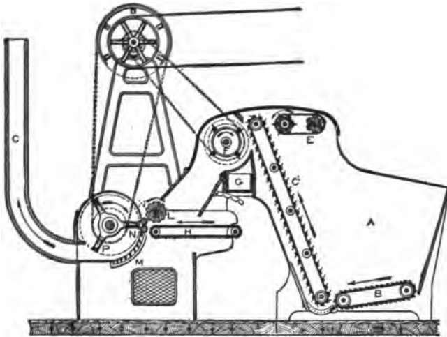
COTTON OPENER AND PICKER
